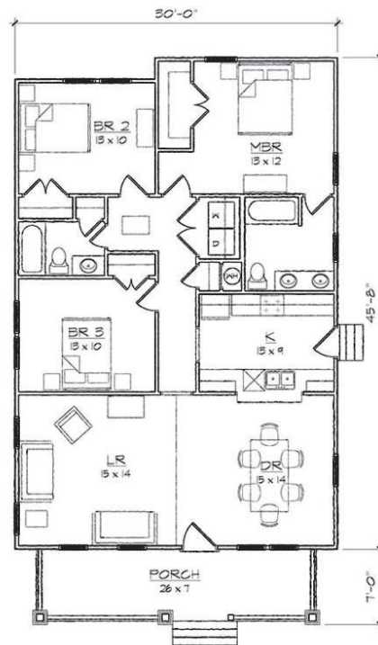
FLOOR PLAN
